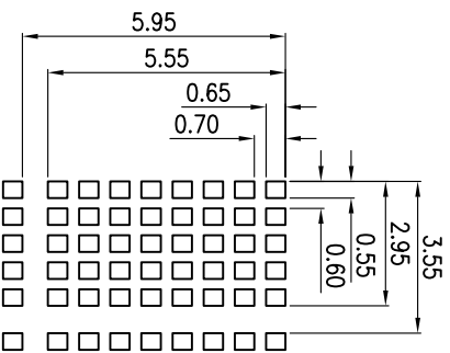
DISPLAY PATTERN
